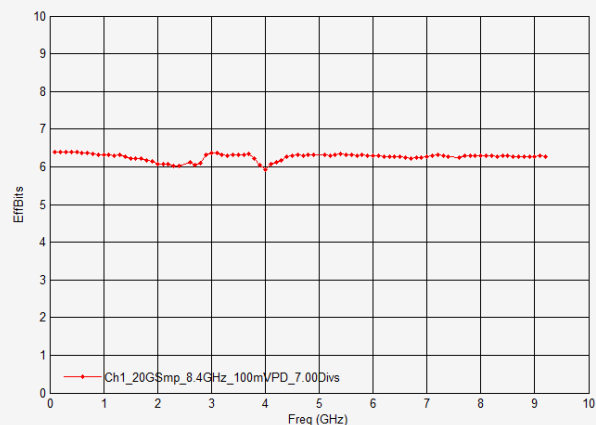
ENOB plot for 8 GHz DSOS804A oscilloscope
