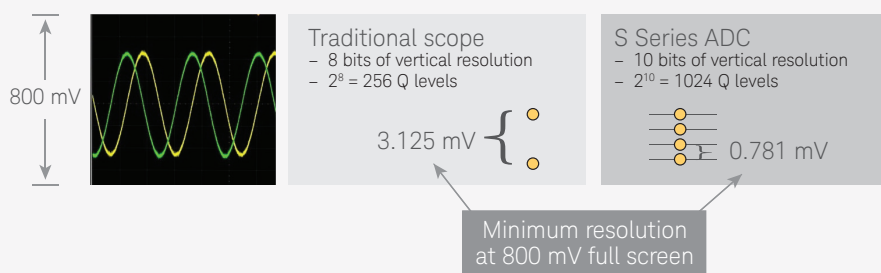
Figure 3. Resolution is an important signal integrity attribute. Having a scope with more ADC bits, and proper vertical scaling are two ways to increase resolution.
