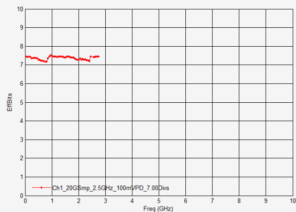
ENOB plot for 2.5 GHz DSOS254A oscilloscope
